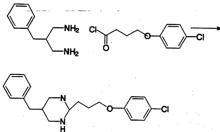
Compound Q
